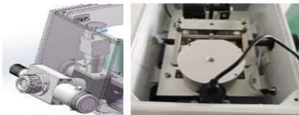
Precision Manual measuring eyepiece (10X) Resolution 0.5µm
